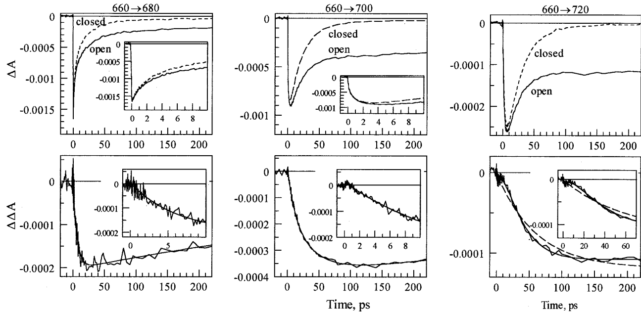
FIGURE 5 Isotropic absorption difference profiles for 660 → 680, 660 → 700, and 660 → 720 nm pump-probe experiments. Top row shows signals for open (solid) and closed (dashed) reaction centers; bottom row shows (open-closed) difference signal. Smooth curves show optimized fits to the difference signals (Table 1). Insets show signal on expanded time scales.
