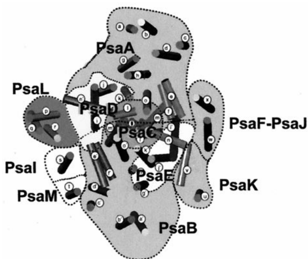
FIGURE 1 Arrangement of protein subunits in the core antenna-reaction center complex of cyanobacterial photosystem I, according to 4 Å structure of Krauss et al. (1995), with subsequent modifications. The reaction center cofactors lie at the boundary between the PsaA and PsaB subunits, directly below subunit PsaC.
