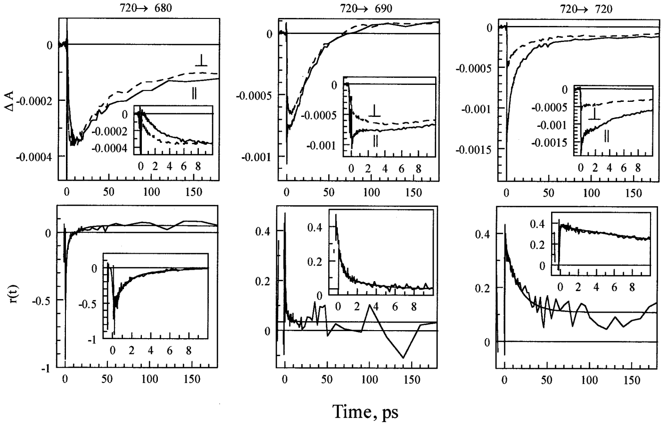
FIGURE 7 Polarized pump-probe profiles \Delta A_{||}(t) , \Delta A_{\perp}(t) and anisotropies r(t) for PS I with open reaction centers, excited at 720 nm. Unlike isotropic signals (Fig. 6), the anisotropies show little dependence on the reaction center oxidation state.
